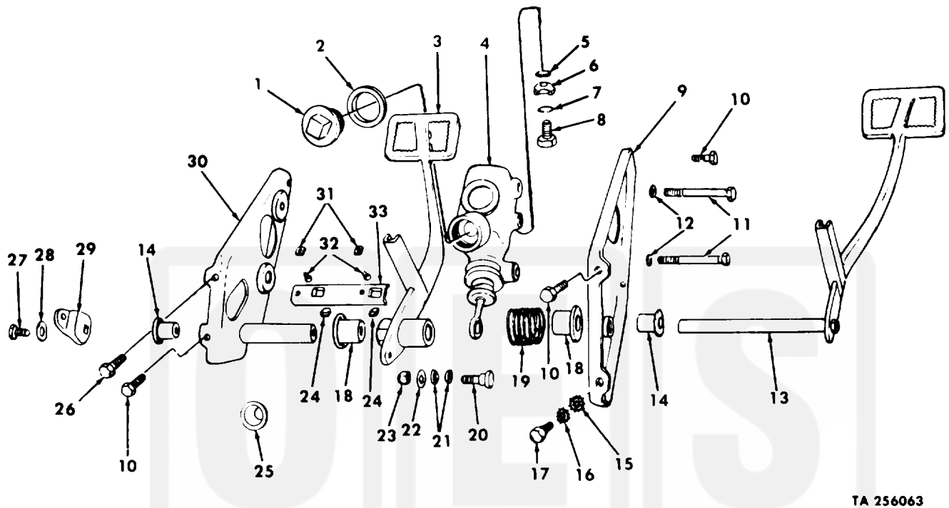
Figure 84. Master Cylinder, Brake Pedal Assembly, and Related Parts. (M151, M151A1, M151A1C, and M718 only).
